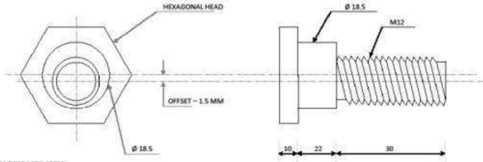
SPECIAL BOLT MOC-SS304
