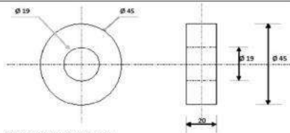
TRAVELLING ROLLER MOC-SS304
