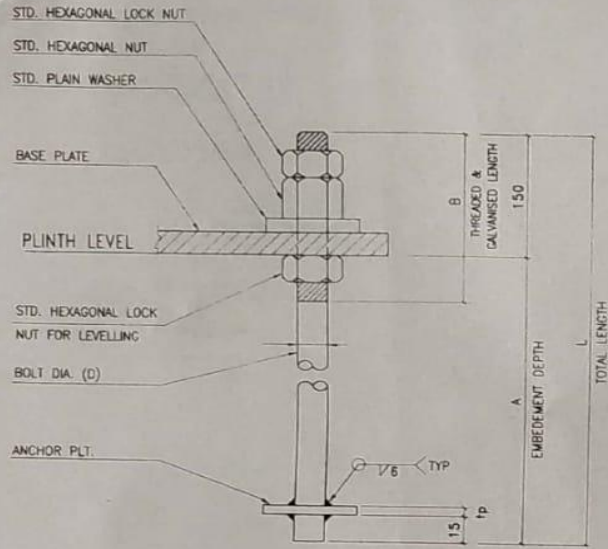
FOUNDATION BOLT
